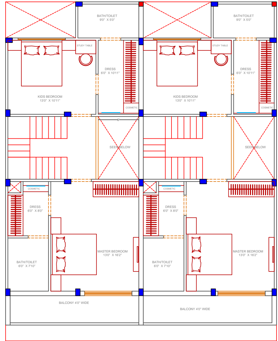
FIRST FLOOR LAYOUT
